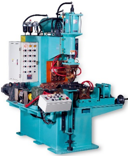
Brake Shoe Projection Seam Welding Machine (Automobile & Truck)
