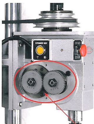
CHANGE THREAD-PITCH GEAR 牙距齒輪更換
