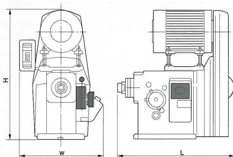
Dimensional Drawing 臥式攻牙機尺寸圖
