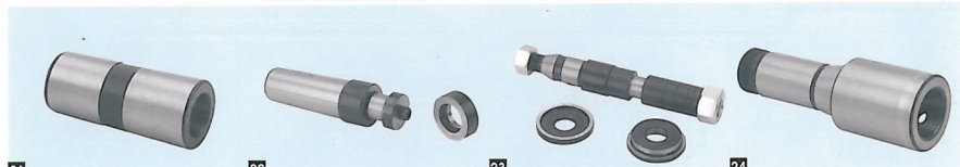
21: TAPER SLEEVES B&S No.11 taper O.D. These sleeves can be used on all types of cutters with taper shanks. AC20 4MT I.D. AC22 2MT I.D. AC21 3MT I.D. AC23 1MT I.D.
