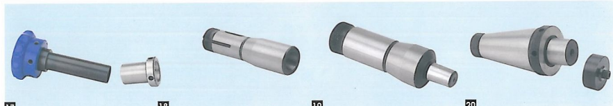
17: COLLET FIXTURE AC01A for changing C2SH from B&S No.11 taper to accept 5C collet. AC01C for changing C2TH from B&S No.11 taper to accept 5C collet.
